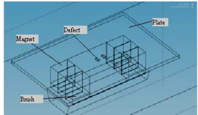
Fig. 2 3D Finite element modeling
