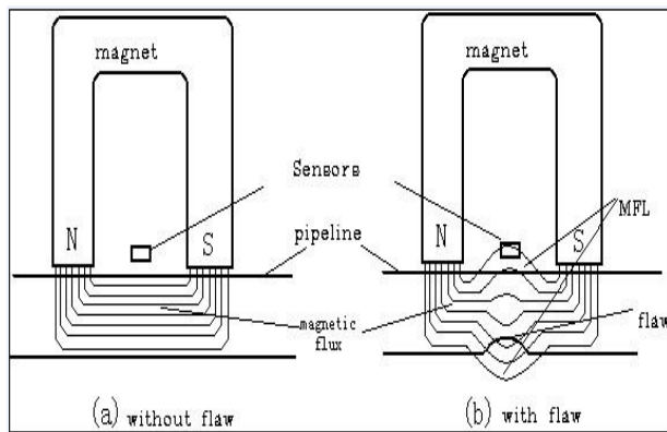
Fig. 1 Components of MFL
