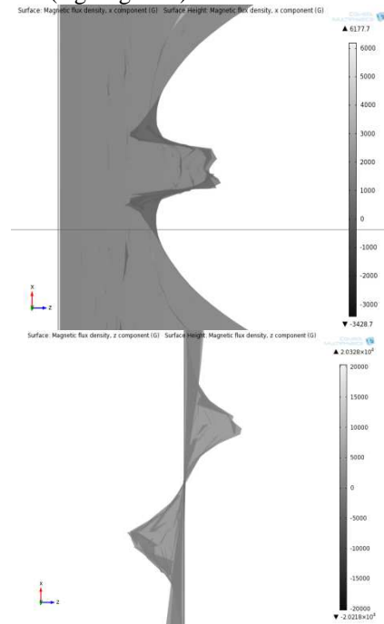
Fig. 4 Graph indicating axial and radial component
